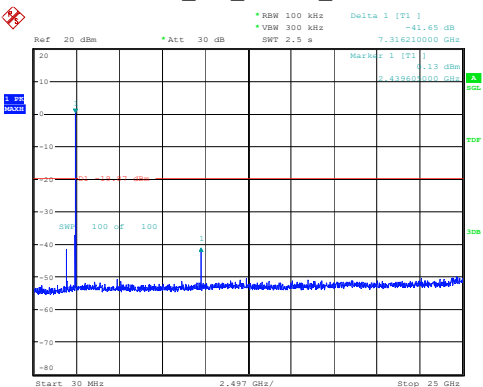
BLE_2M_Middle_Channel
