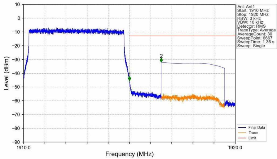
Band25_5MHz_16QAM_HCH_1912.5MHz_RB_1_24_NTNV
