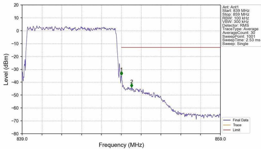
Band26b_10MHz_QPSK_HCH_844MHz_RB_50_0_NTNV
