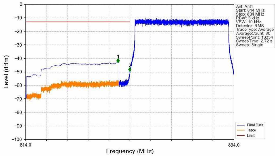
Band26b_10MHz_16QAM_LCH_829MHz_RB_1_0_NTNV
