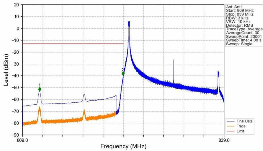
Band26b_15MHz_16QAM_LCH_831.5MHz_RB_1_0_NTNV
