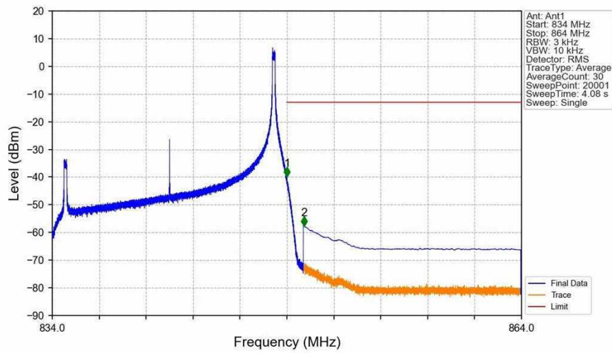
Band26b_15MHz_16QAM_HCH_841.5MHz_RB_1_74_NTNV
