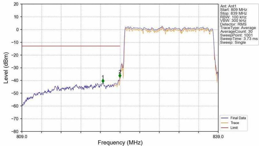
Band26b_15MHz_16QAM_LCH_831.5MHz_RB_75_0_NTNV
