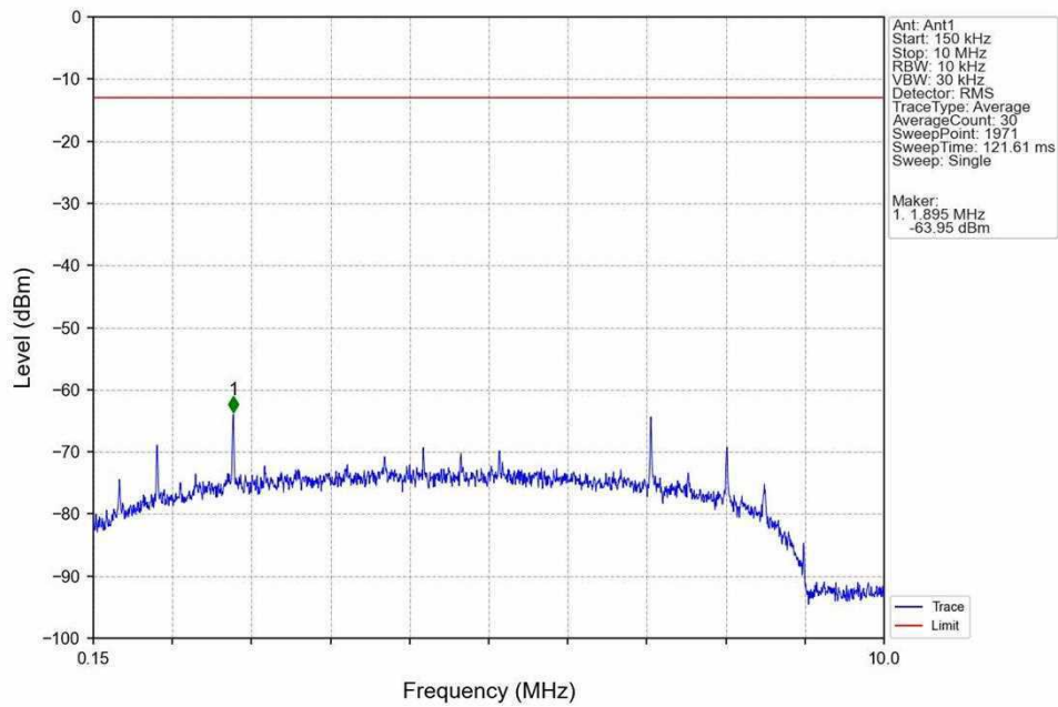
Band66_10MHz_16QAM_HCH_1775MHz_RB_1_0_NTNV
