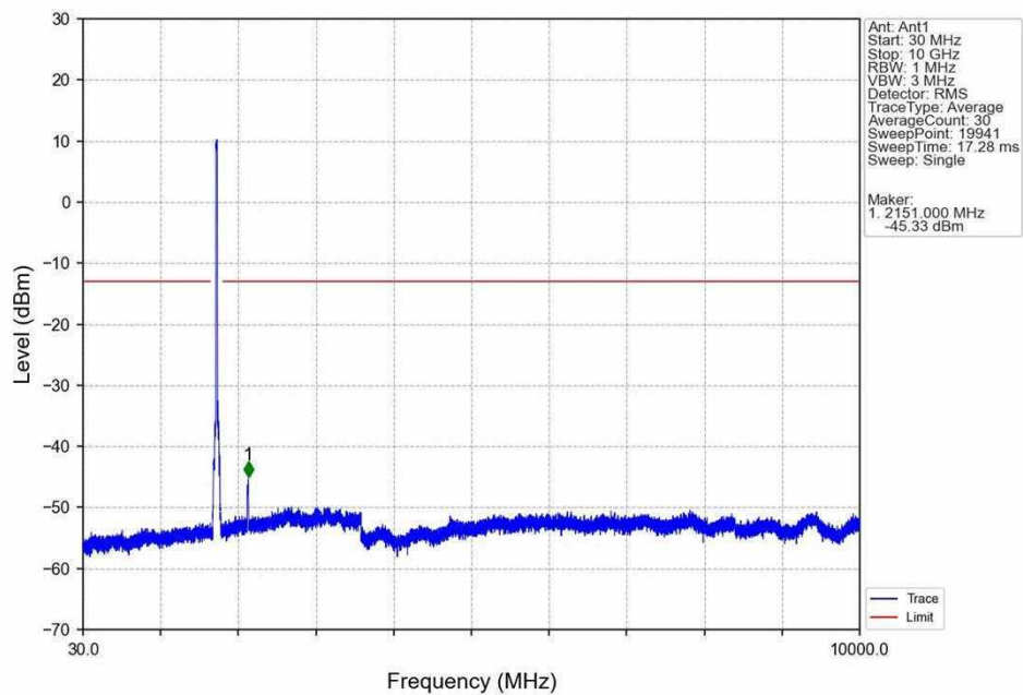
Band66_20MHz_16QAM_MCH_1745MHz_RB_1_0 NTN
