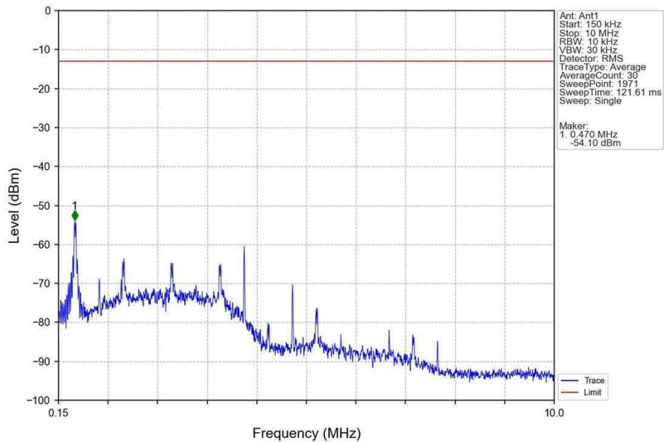
Band5_HSUPA_HCH_846.6MHz_Subtest 1_NTNV
