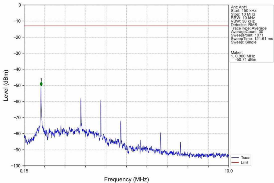
Band5_HSDPA_HCH_846.6MHz_Subtest 1_NTNV
