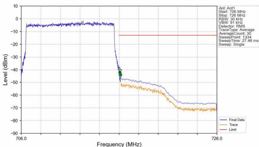
Band12_10MHz_16QAM_HCH_711MHz_RB_50_0_NTNV
