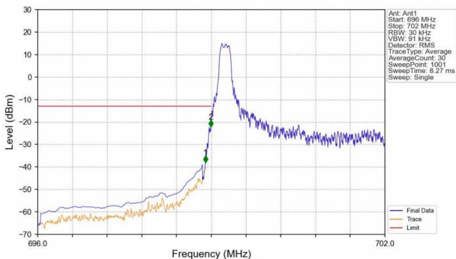
Band12_3MHz_16QAM_LCH_700.5MHz_RB_1_0_NTNV
