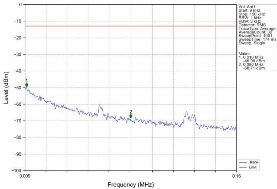
Band12_3MHz_QPSK_HCH_714.5MHz_RB_1_0_NTNV
