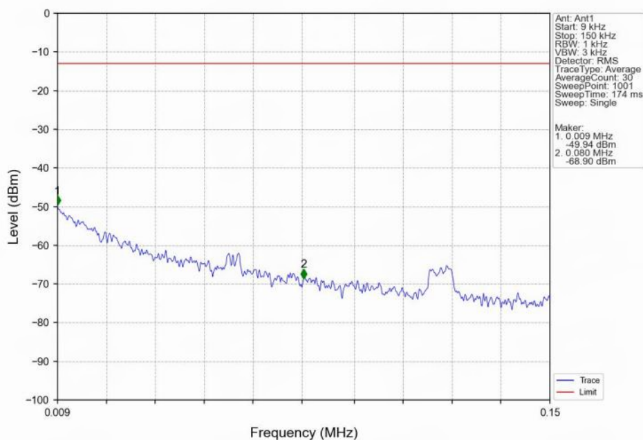
Band12_3MHz_16QAM_LCH_700.5MHz_RB_1_0_NTNV
