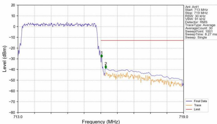
Band12_3MHz_QPSK_HCH_714.5MHz_RB_15_0_NTNV
