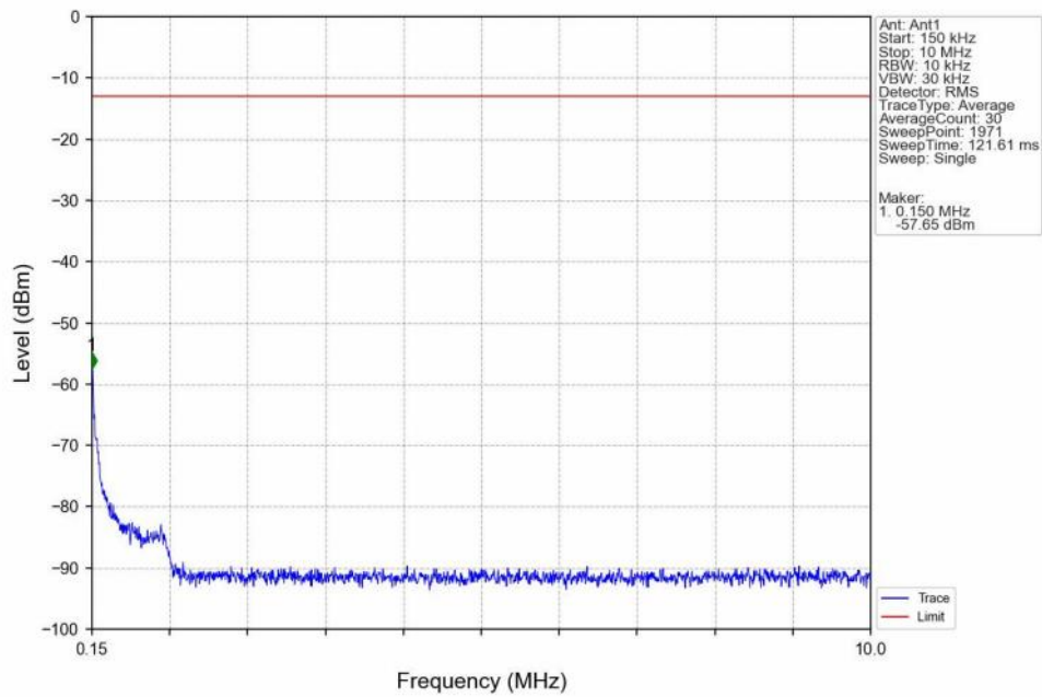
Band12_1.4MHz_16QAM_LCH_699.7MHz_RB_1_0_NTNV
