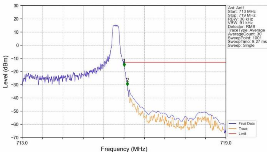
Band12_3MHz_QPSK_HCH_714.5MHz_RB_1_14_NTNV
