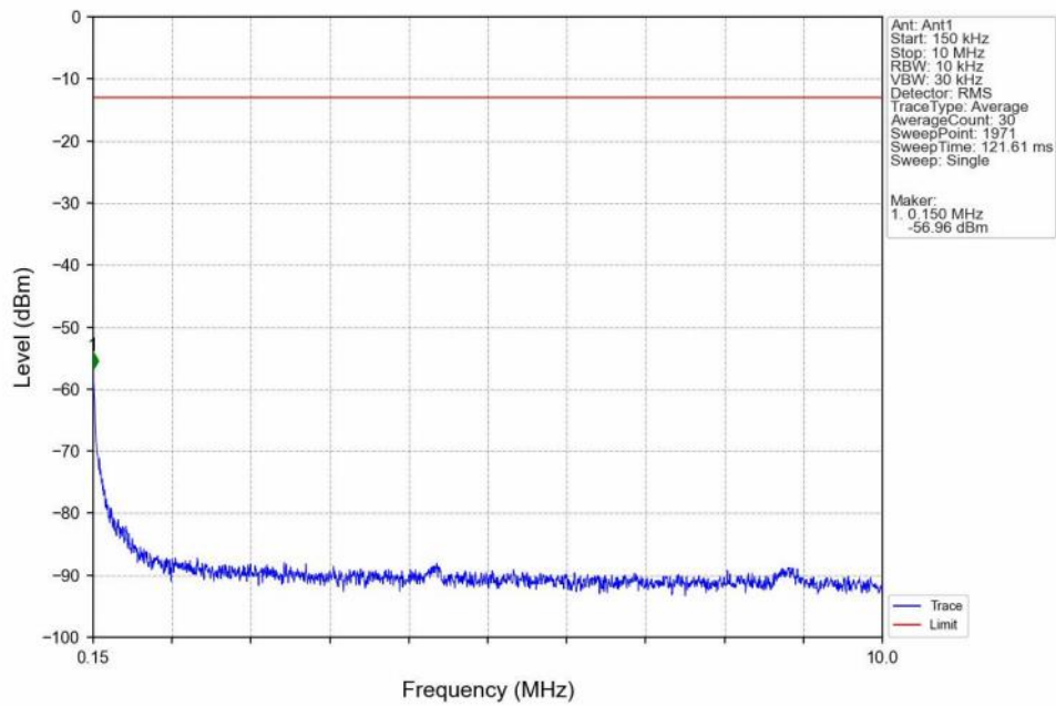
Band12_10MHz_16QAM_LCH_704MHz_RB_1_0_NTNV
