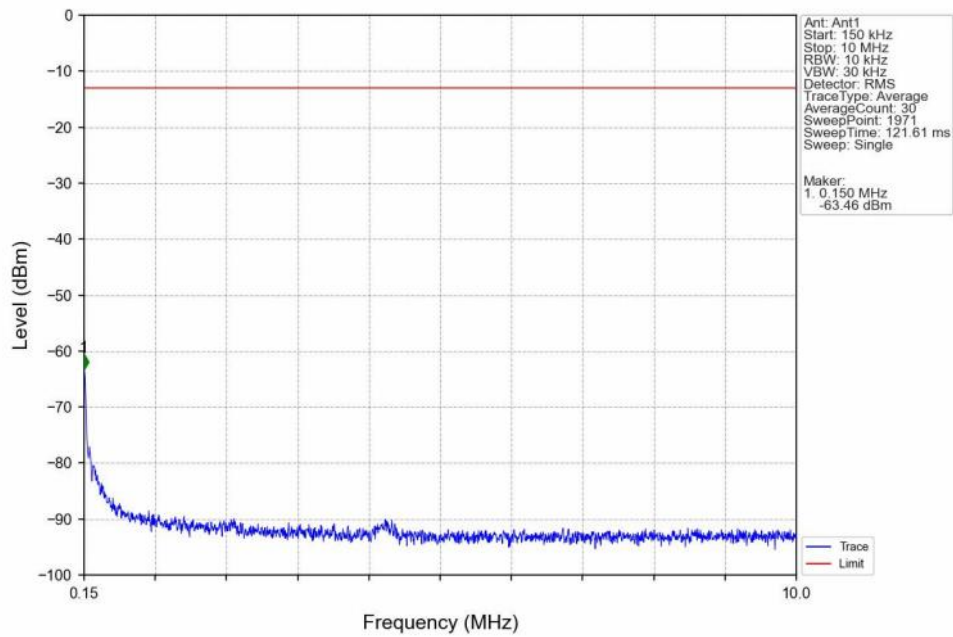
Band25_5MHz_16QAM_HCH_1912.5MHz_RB_1_0_NTNV
