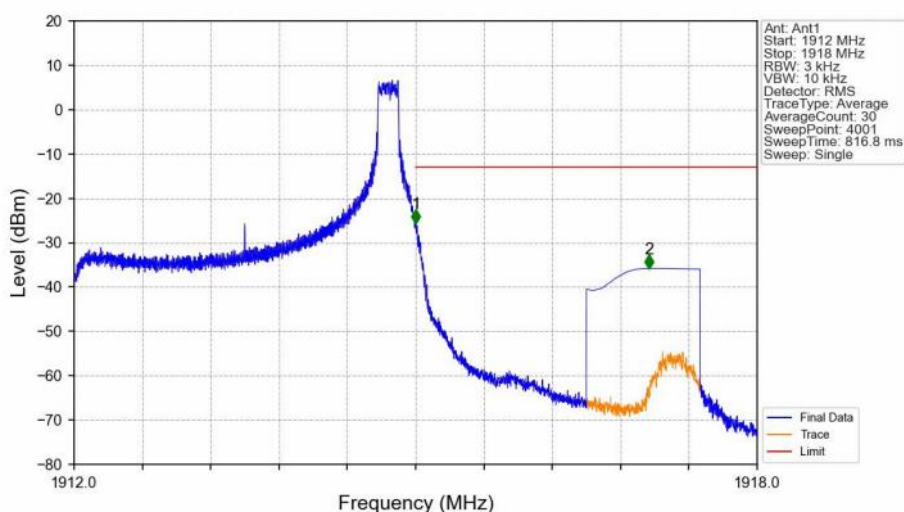
Band25_3MHz_QPSK_HCH_1913.5MHz_RB_1_14_NTNV
