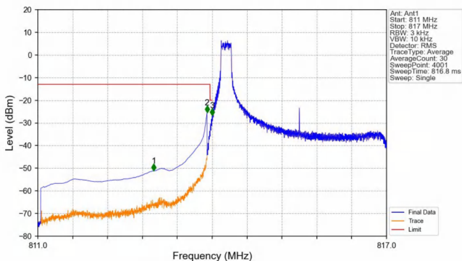
Band26a_3MHz_16QAM_LCH_815.5MHz_RB_1_0_NTNV
