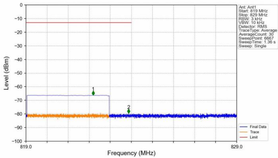
Band26b_5MHz_16QAM_LCH_826.5MHz_RB_1_0_NTNV
