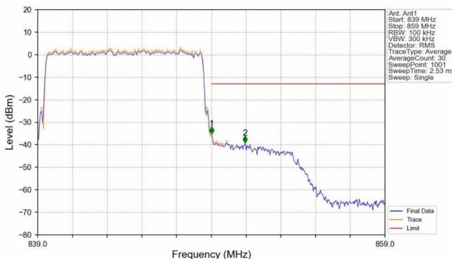
Band26b_10MHz_16QAM_HCH_844MHz_RB_50_0_NTNV
