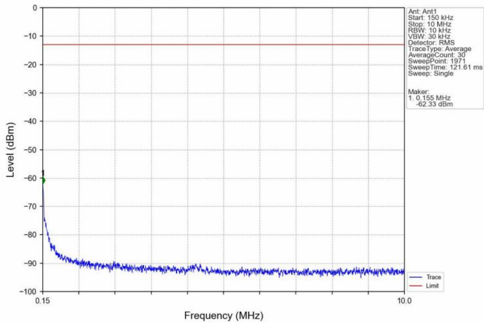
Band4_5MHz_16QAM_HCH_1752.5MHz_RB_1_0_NTNV
