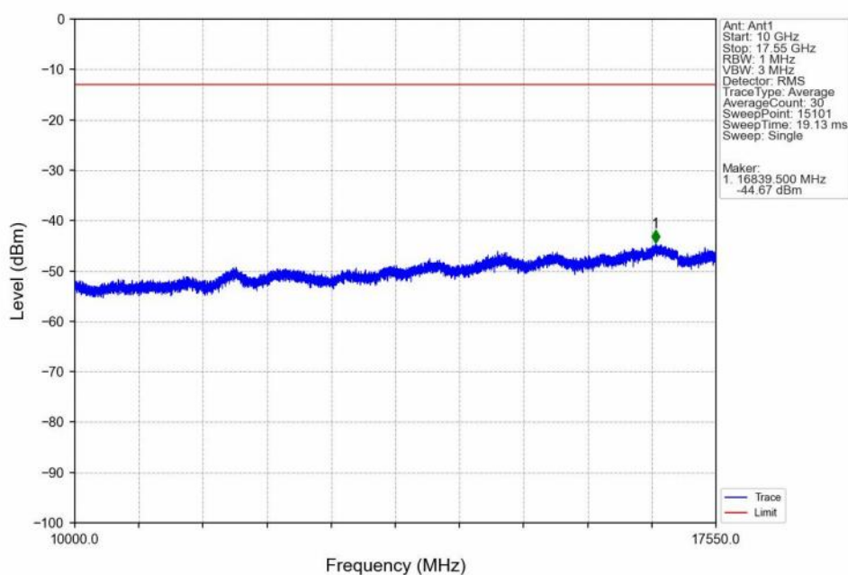
Band4_10MHz_QPSK_LCH_1715MHz_RB_1_0_NTNV
