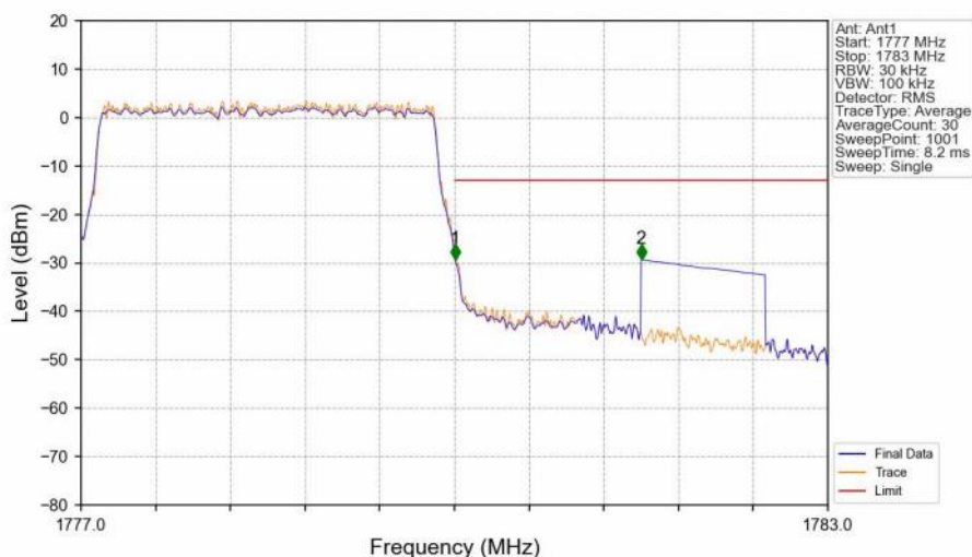
Band66_3MHz_16QAM_HCH_1778.5MHz_RB_15_0_NTNV
