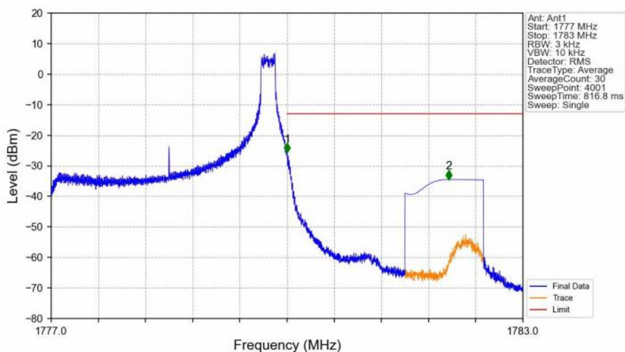
Band66_3MHz_16QAM_HCH_1778.5MHz_RB_1_14_NTNV
