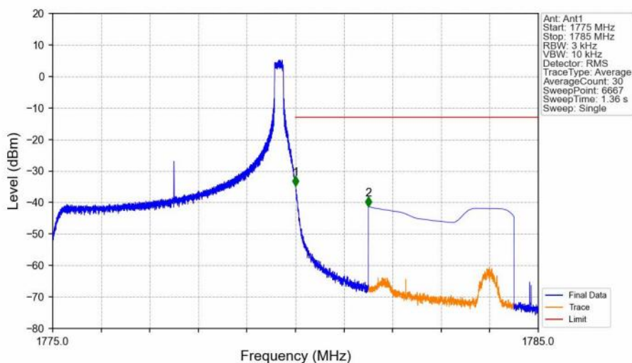
Band66_5MHz_16QAM_HCH_1777.5MHz_RB_1_24_NTNV
