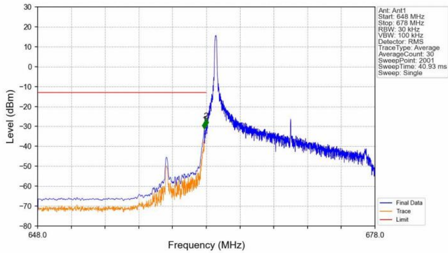
Band71_15MHz_16QAM_LCH_670.5MHz_RB_1_0_NTNV
