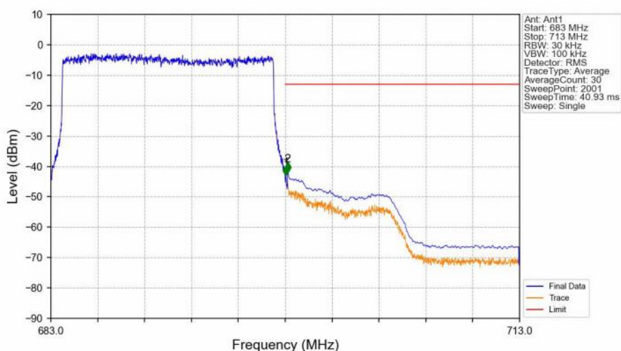
Band71_15MHz_QPSK_HCH_690.5MHz_RB_75_0_NTNV
