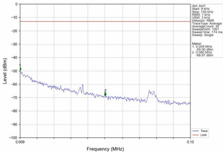
Band71_15MHz_16QAM_LCH_670.5MHz_RB_1_0_NTNV
