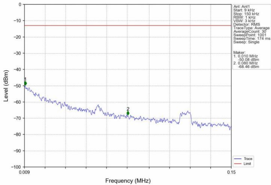
Band71_5MHz_16QAM_HCH_695.5MHz_RB_1_0_NTNV
