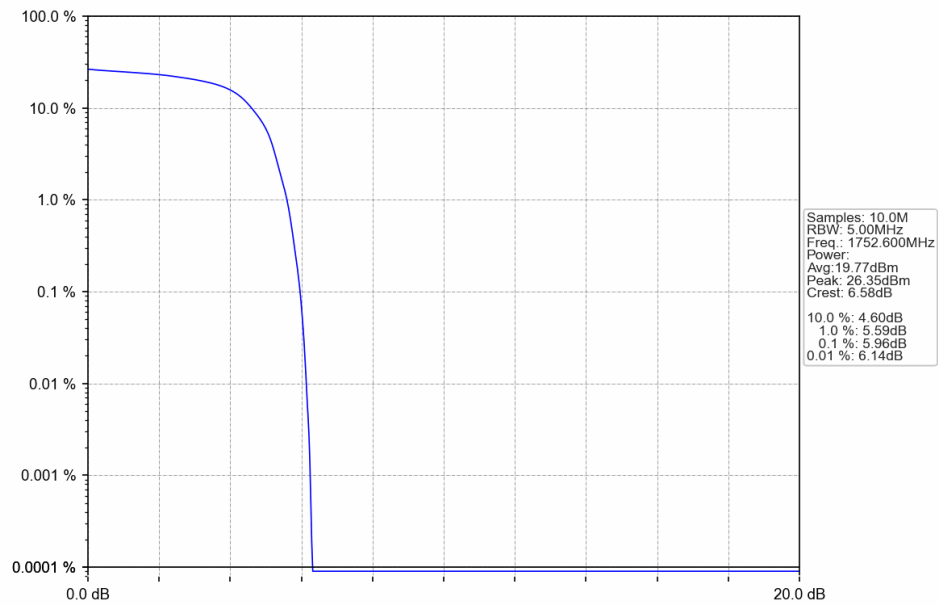
Band4 HSUPA HCH 1752.6MHz Subtest 1 NTN
