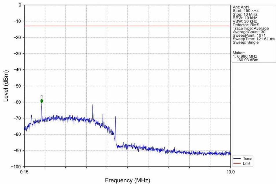
Band12_5MHz_16QAM_HCH_713.5MHz_RB_1_0_NTNV
