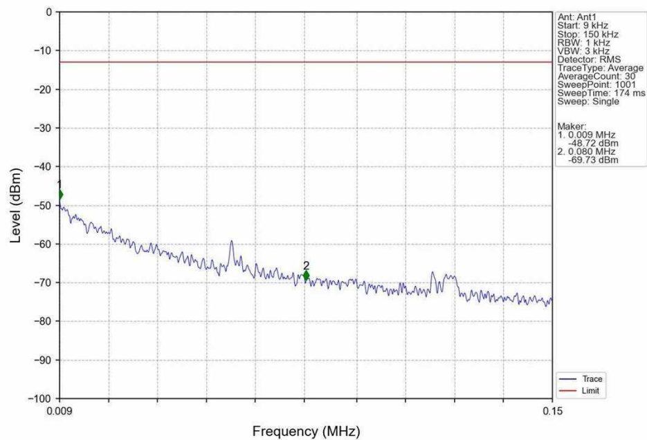
Band12_10MHz_16QAM_LCH_704MHz_RB_1_0_NTNV
