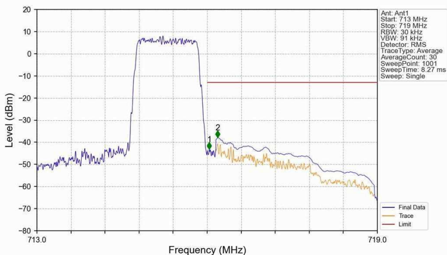
Band12_1.4MHz_16QAM_HCH_715.3MHz_RB_1_5_NTNV
