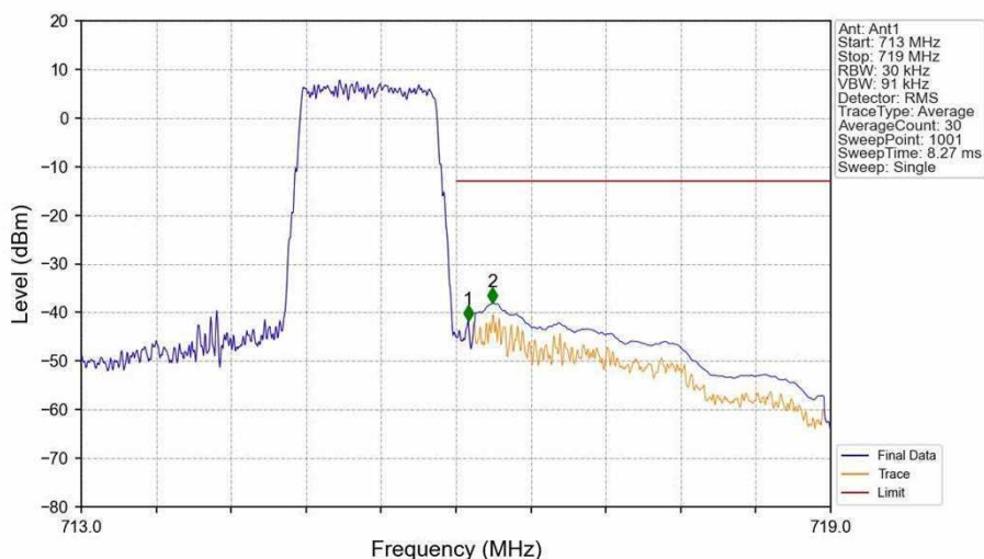
Band12_1.4MHz_16QAM_HCH_715.3MHz_RB_6_0_NTNV
