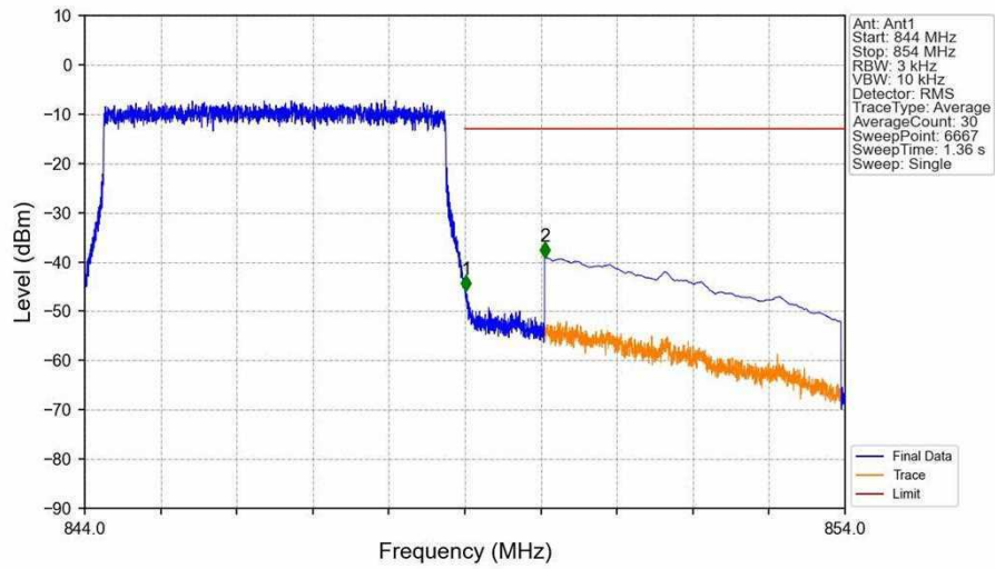
Band5_5MHz_16QAM_HCH_846.5MHz_RB_1_24_NTNV
