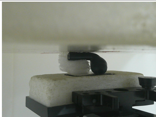
Photo 10: Top Side_Right Earphone_0mm
