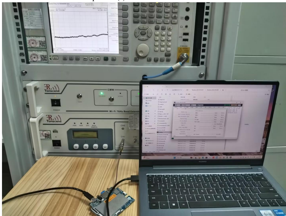
Test Setup Photo(s) of RF Conducted Measurement
