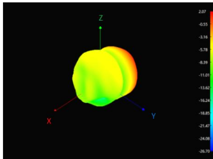
2440MHz 3D
