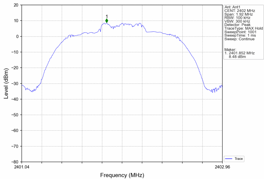
Pi/4DQPSK_2DH5_LCH_2402MHz_Ant1_NTNV
