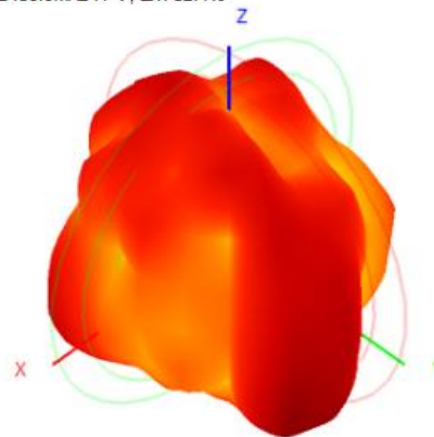
2450.0MHz H+V, Eff: 52.4%
