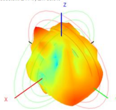
5850.0MHz H+V, Eff: 53.8%
