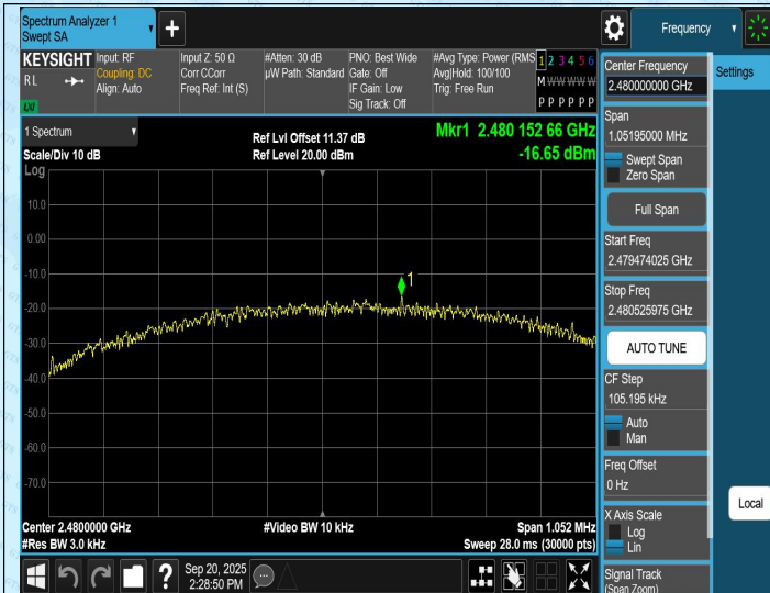
BLE_1M-Ant1-2480-PASS
