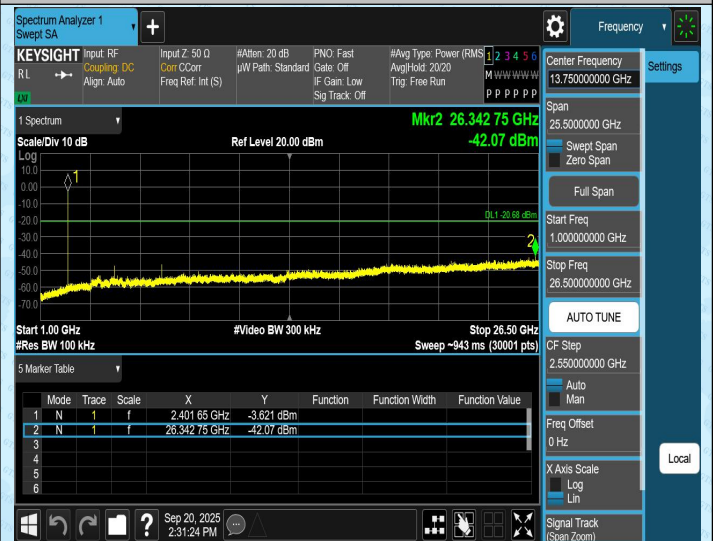
BLE_2M-Ant1-2402-1000~26500-PASS
