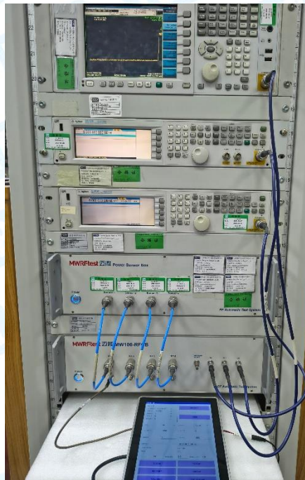
Photo of Setup for Conducted Measurements
