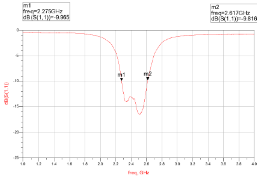
Figure 5: Measured S11, Full Size IFA
