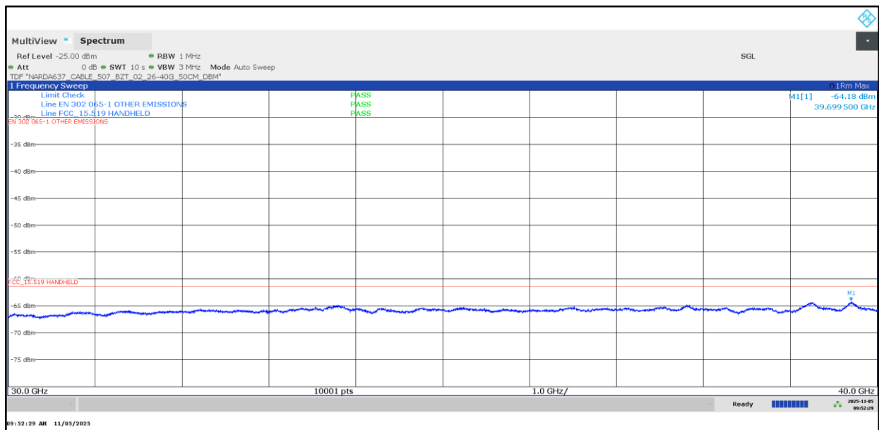
Plot 10: 30 GHz to 40.0 GHz, UWB test mode
