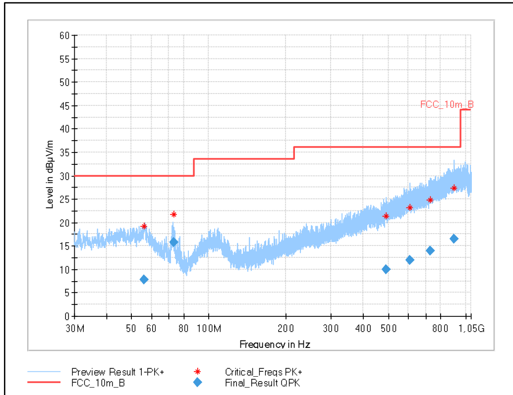
Plot 5: 30 MHz to 1 GHz, UWB test mode
