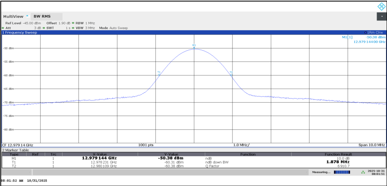
Plot 13: 13 GHz spurious emission: EUT 1; RBW 1MHz; TX on
