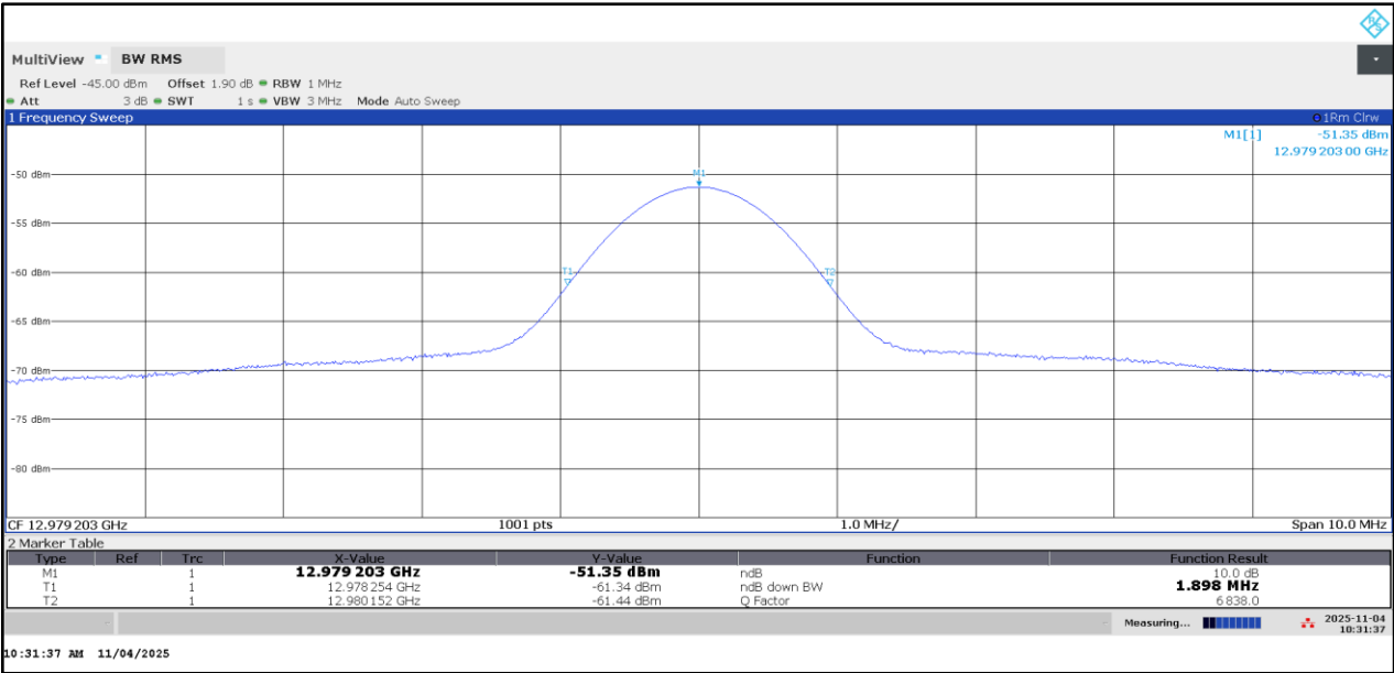
Plot 15: 13 GHz spurious emission: EUT 2; RBW 1 MHz; TX on
