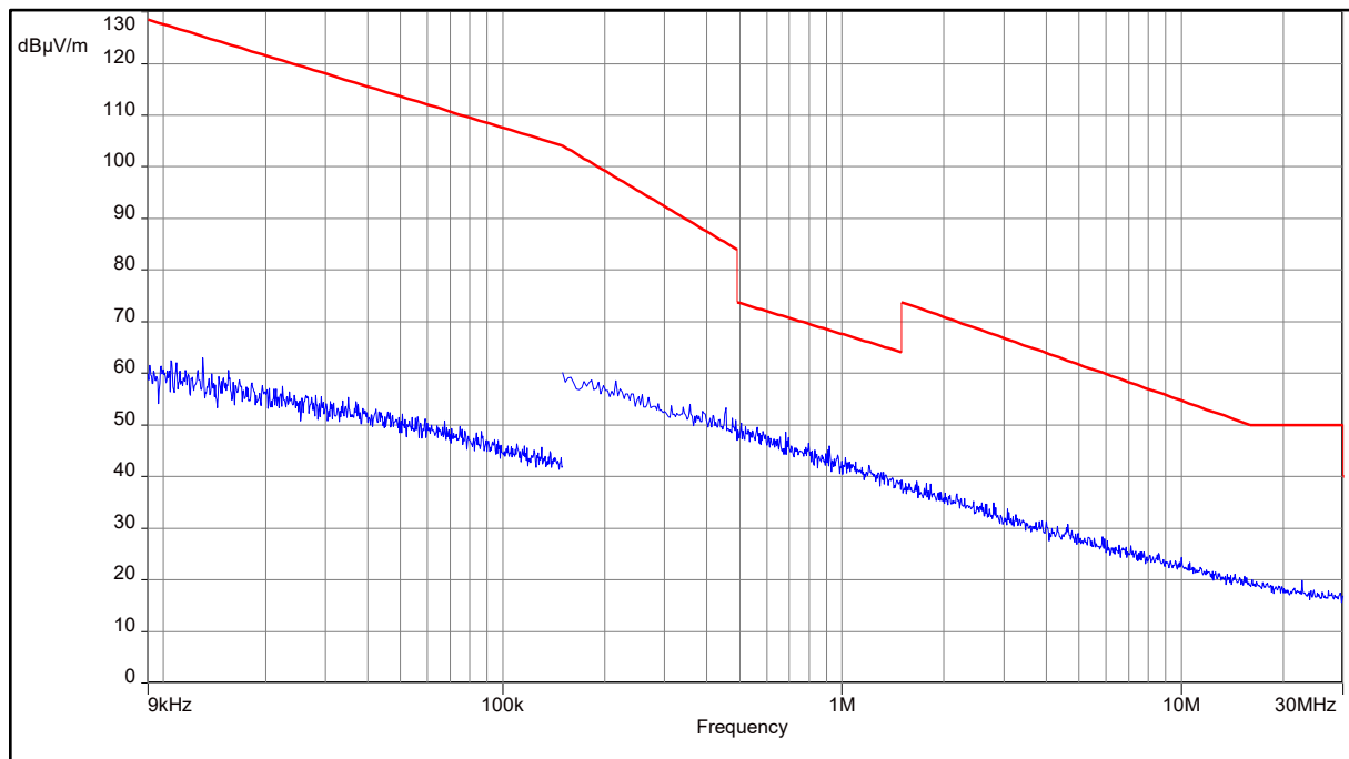
Plot 4: 9 kHz to 30 MHz, UWB test mode
