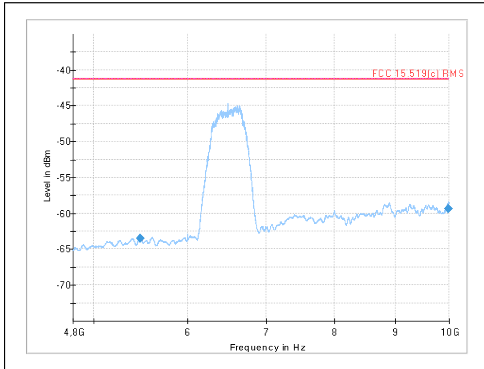
Plot 7: 4.8 GHz to 10 GHz, UWB test mode
