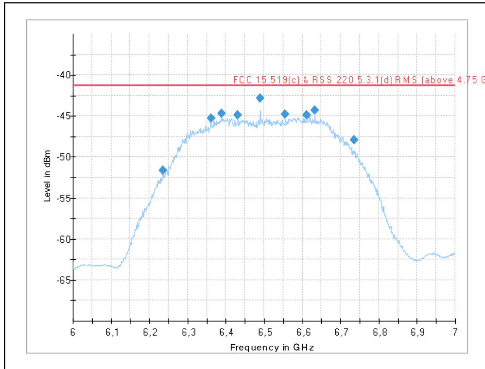
Plot 2: Fundamental emission (UWB test mode): RMS
