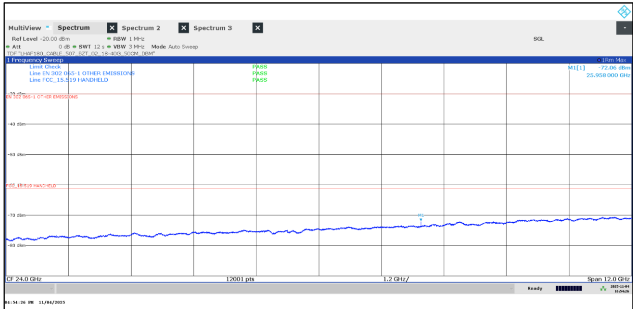
Plot 9: 18 GHz to 30 GHz, UWB test mode
