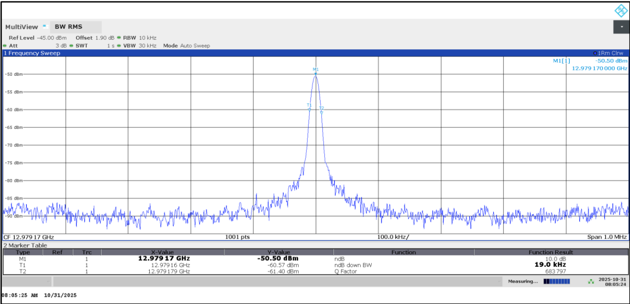
Plot 19: 13 GHz spurious emission: EUT 1; RBW 10kHz; TX on
