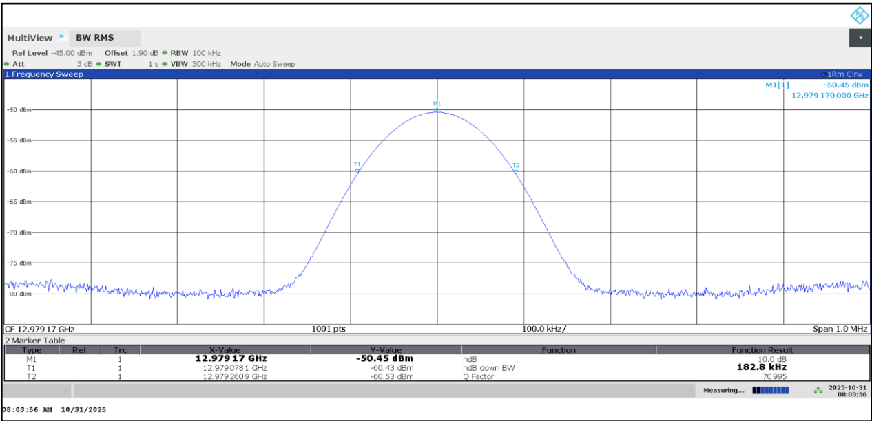
Plot 16: 13 GHz spurious emission: EUT 1; RBW 100kHz; TX on
