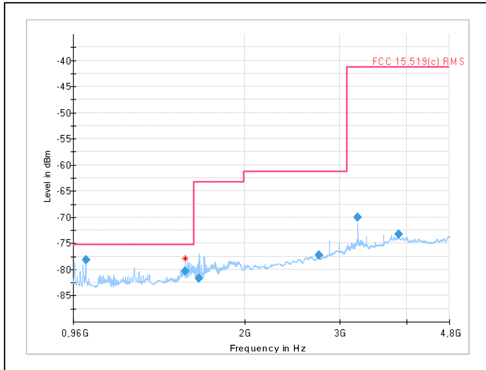
Plot 6: 960 MHz to 4.8 GHz (Limit acc. to §15.519 (c)), UWB test mode
