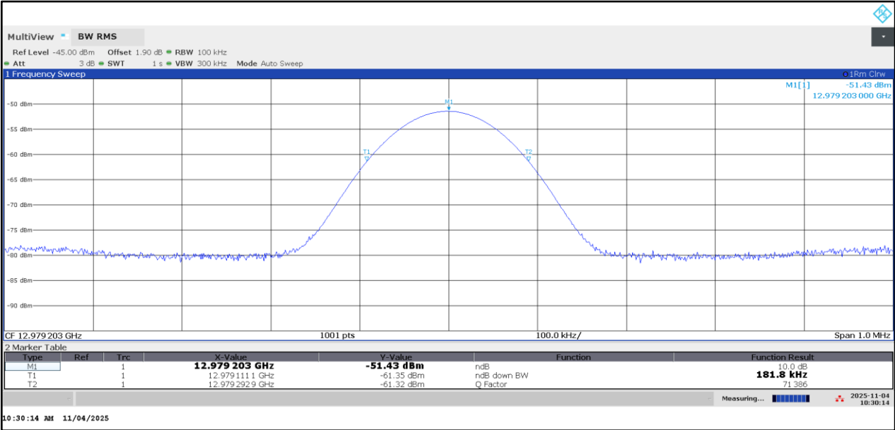
Plot 18: 13 GHz spurious emission: EUT 2; RBW 100kHz; TX on
