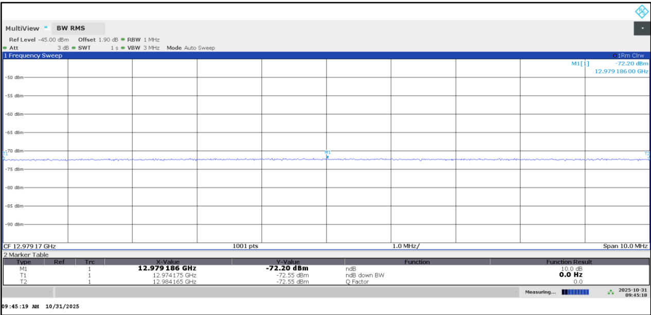
Plot 14: 13 GHz spurious emission: EUT 1; RBW 1MHz; UWB module off
