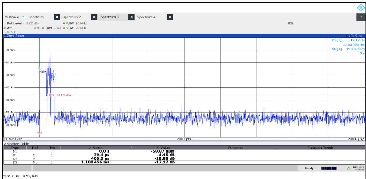
Plot 24: Emission of EUT without an associated receiver over a short timescale; normal mode
