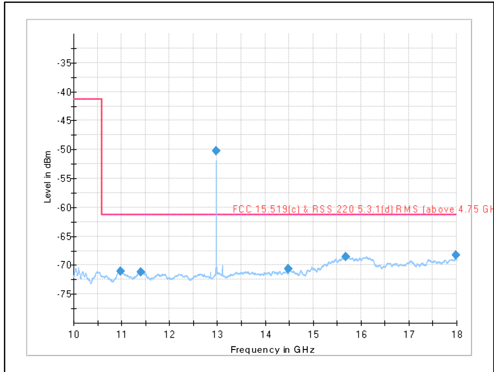
Plot 8: 10 GHz to 18 GHz, UWB test mode
