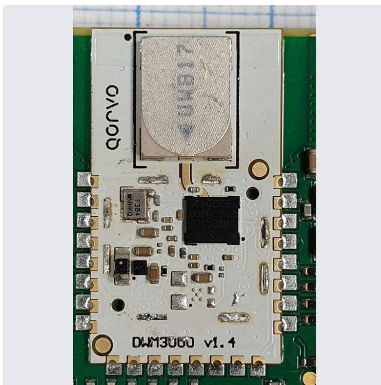
Photo 3 UWB module without shielding cap
