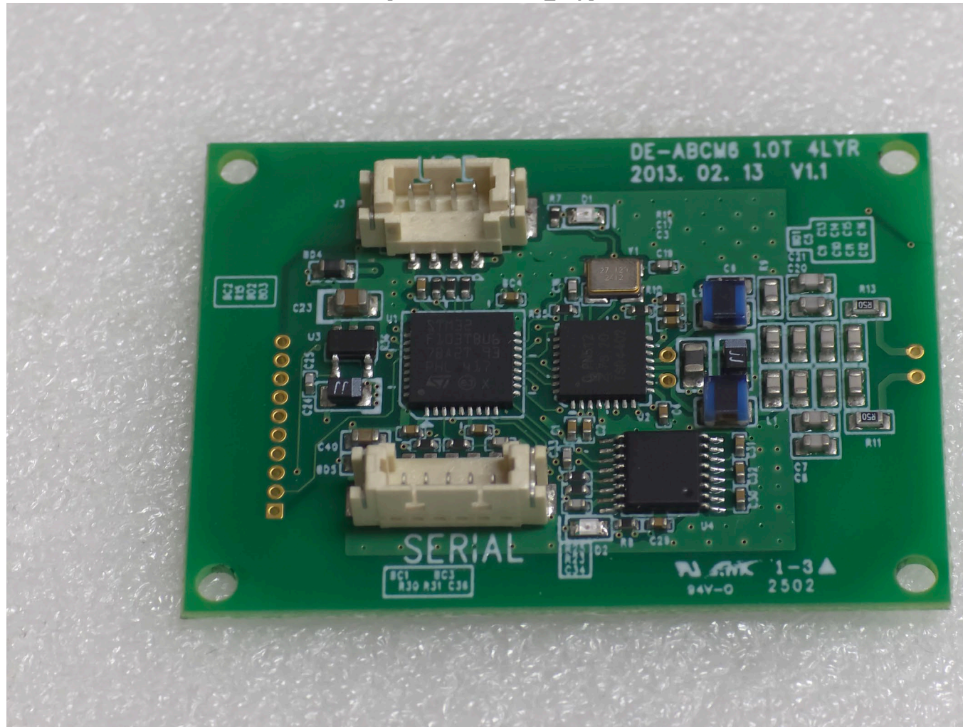
[Sub PCB Board2_Top]
