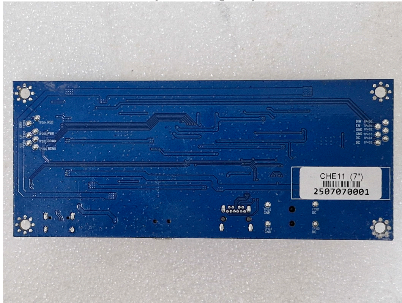
[Main PCB Board_Bottom]
