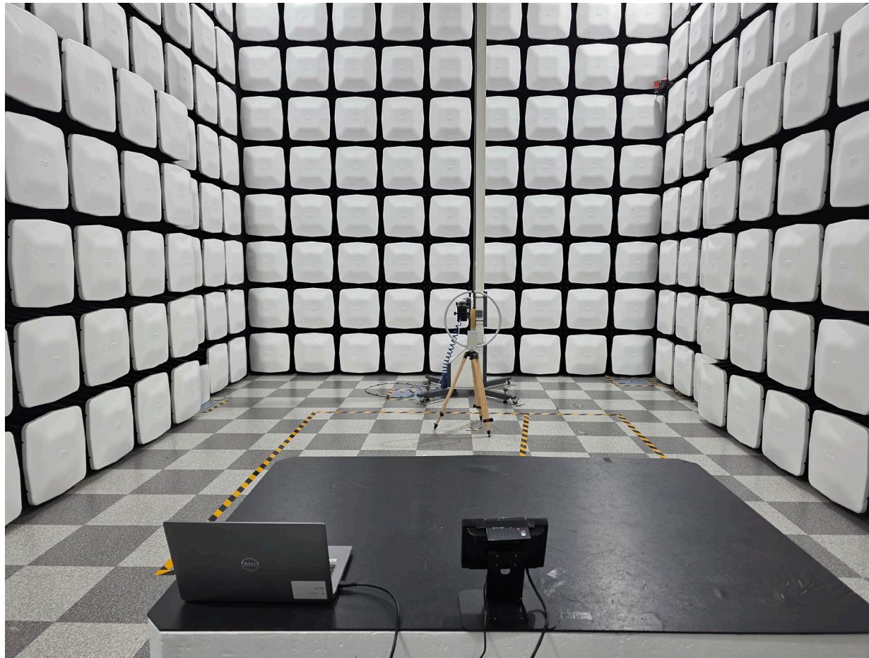
Radiated RF measurement (9 kHz ~ 30 MHz)
