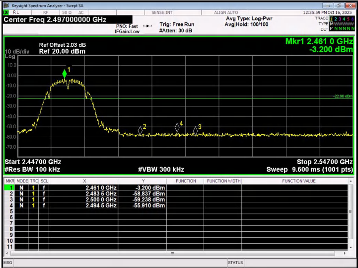
802.11b: Band Edge, Right Side
