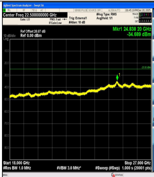
Band41-20MHz-16QAM-41490-1RB#99-0.15~30 -PASS
