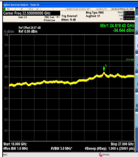
Band41-20MHz-QPSK-41490-100RB#0-0.15~30-PASS
