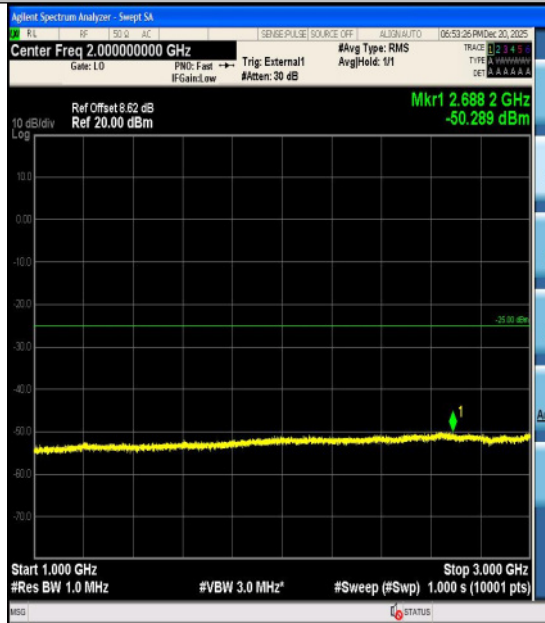
Band41-20MHz-QPSK-41490-100RB#0-18000~ 27000-PASS
