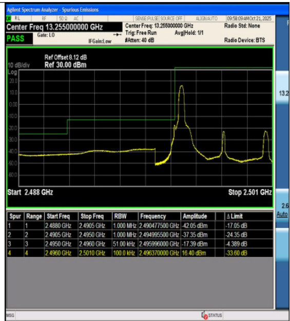
Band41-5MHz-16QAM-39675-25RB#0-PASS
