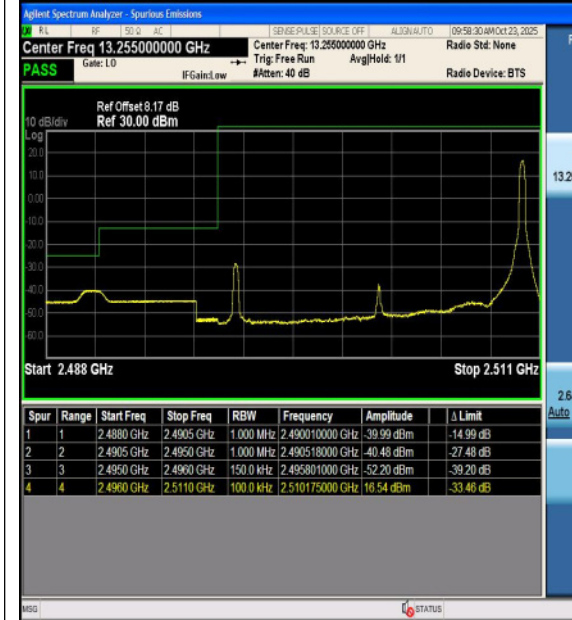
Band41-15MHz-QPSK-41515-1RB#0-PASS
