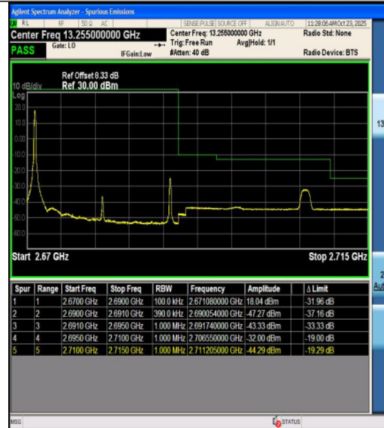
Band41-20MHz-16QAM-41490-100RB#0-PASS
