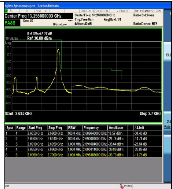
Band41-5MHz-16QAM-41565-1RB#0-PASS
