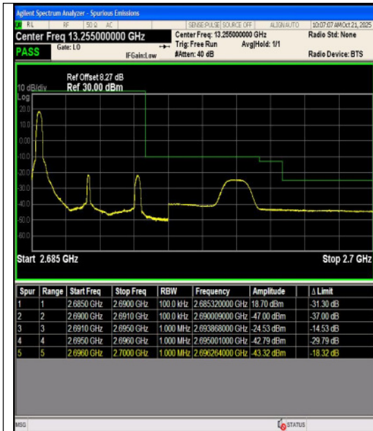
Band41-5MHz-QPSK-41565-25RB#0-PASS
