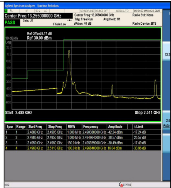
Band41-15MHz-16QAM-39725-75RB#0-PASS
