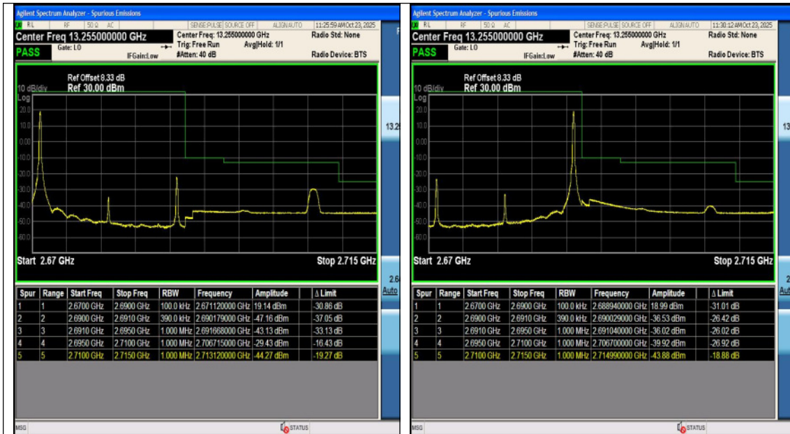
Band41-20MHz-QPSK-41490-100RB#0-PASS
