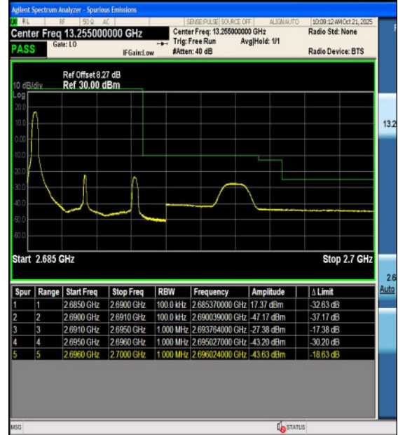
Band41-5MHz-16QAM-41565-25RB#0-PASS
