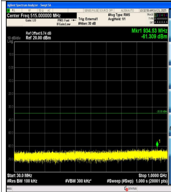
Band41-5MHz-QPSK-40620-1RB#0-3000~1800 0-PASS
