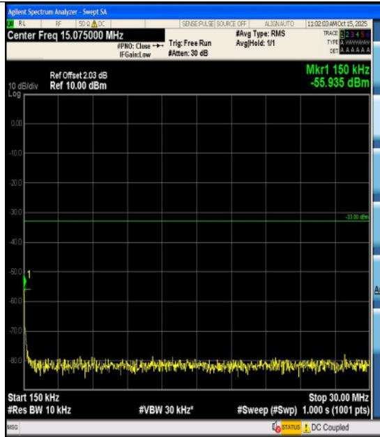
Band4-20MHz-QPSK-20300-1RB#0-1000~3000-P PASS
