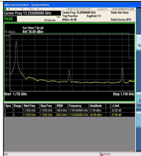
Band4-20MHz-16QAM-20300-100RB#0-PASS
