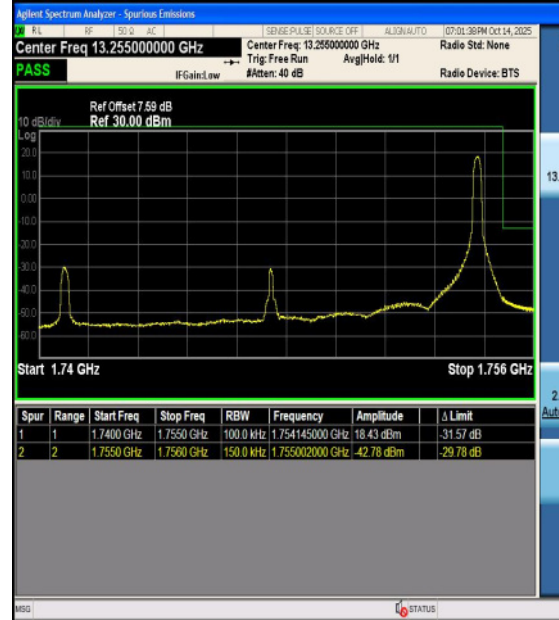
Band4-15MHz-16QAM-20325-1RB#0-PASS
