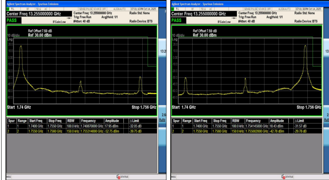
Band4-15MHz-QPSK-20325-75RB#0-PASS
