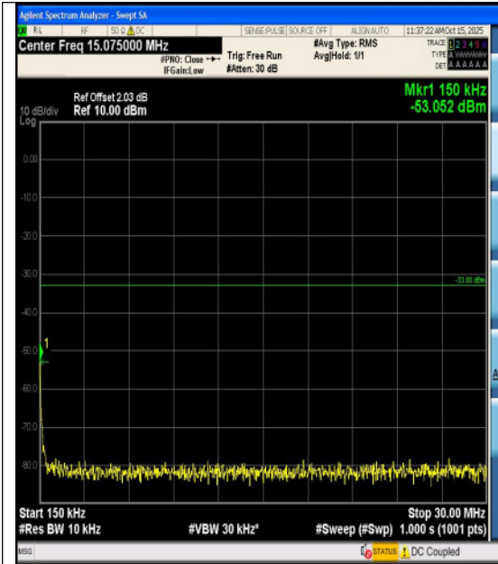
Band4-1.4MHz-QPSK-19957-1RB#5-1000~3000 -PASS
