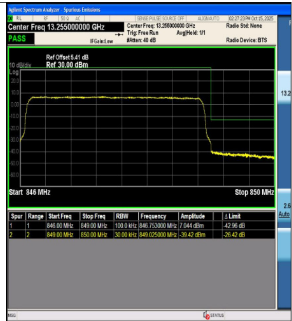
Band5-5MHz-QPSK-20425-1RB#24-PASS
