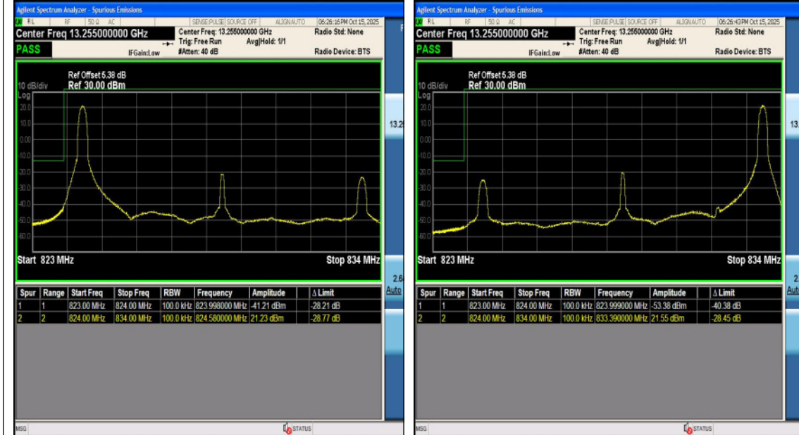
Band5-10MHz-QPSK-20450-50RB#0-PASS
