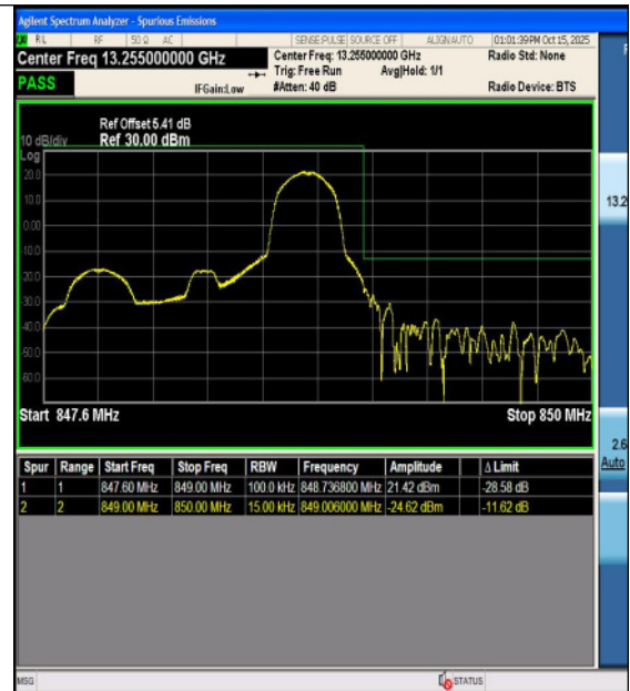
Band5-1.4MHz-16QAM-20643-1RB#0-PASS
