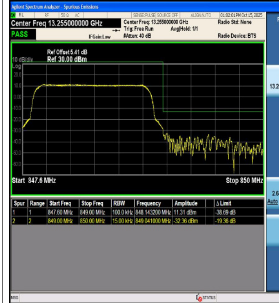
Band5-1.4MHz-16QAM-20643-1RB#5-PASS
