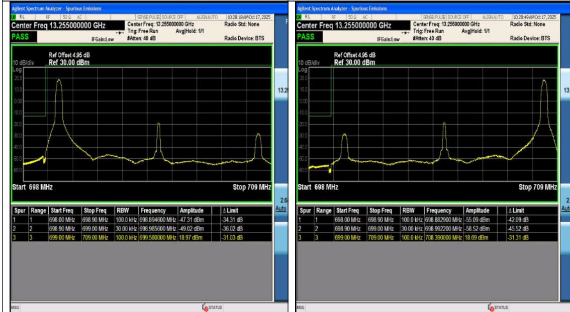
Band12-10MHz-QPSK-23060-50RB#0-PASS
