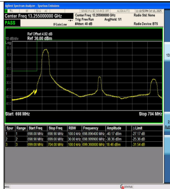
Band12-5MHz-16QAM-23035-25RB#0-PASS
