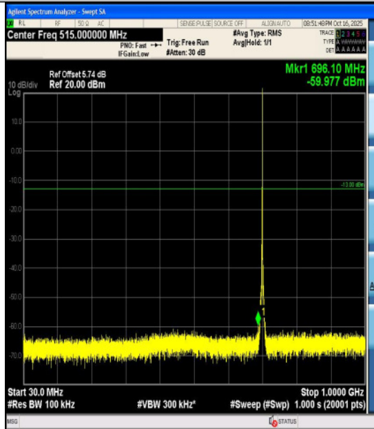
Band12-1.4MHz-QPSK-23095-1RB#5-3000~100 00-PASS
