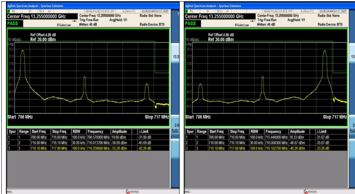
Band12-10MHz-QPSK-23130-50RB#0-PASS
