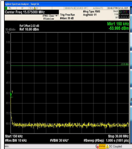
Band12-1.4MHz-16QAM-23017-6RB#0-1000~30 00-PASS
