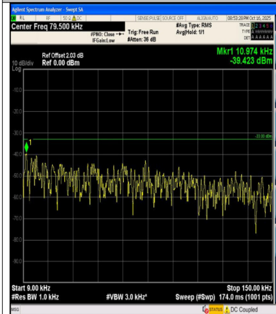
Band12-1.4MHz-QPSK-23095-6RB#0-0~30~1000- PASS
