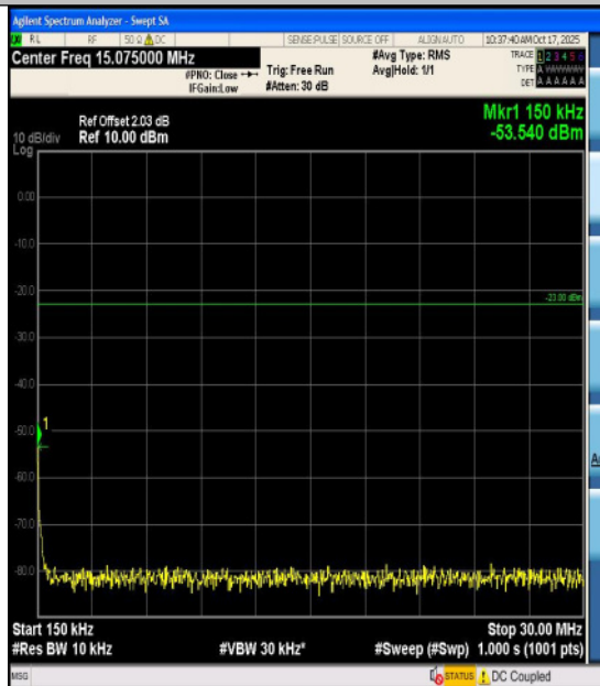
Band12-10MHz-QPSK-23095-1RB#0-1000~300 0-PASS
