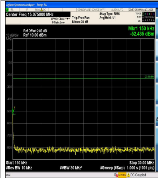
Band12-5MHz-16QAM-23155-1RB#0-1000~300 0-PASS
