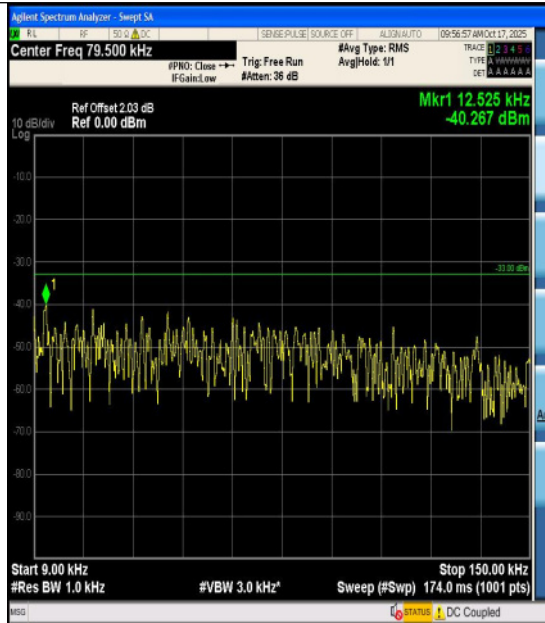
Band12-5MHz-16QAM-23155-1RB#0-30~1000-P ASS
