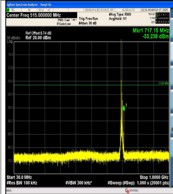
Band12-10MHz-QPSK-23060-1RB#0-3000~100 00-PASS
