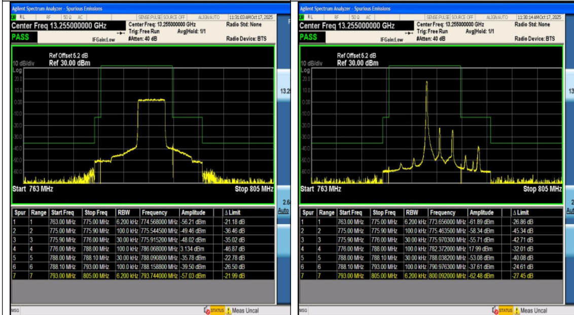
Band13-5MHz-16QAM-23255-1RB#24-PASS
