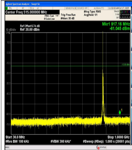
Band13-5MHz-QPSK-23205-1RB#0-3000~1000 0-PASS
