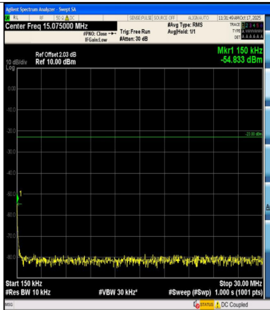
Band13-5MHz-QPSK-23205-1RB#0-1000~3000-P PASS
