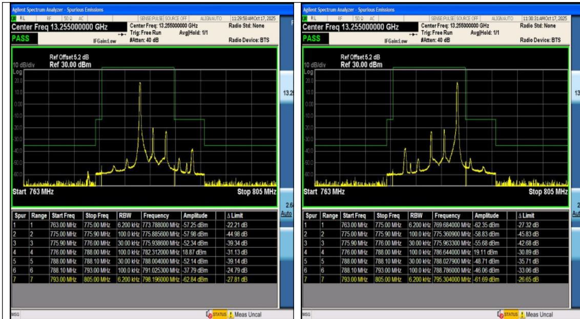
Band13-5MHz-QPSK-23255-25RB#0-PASS
