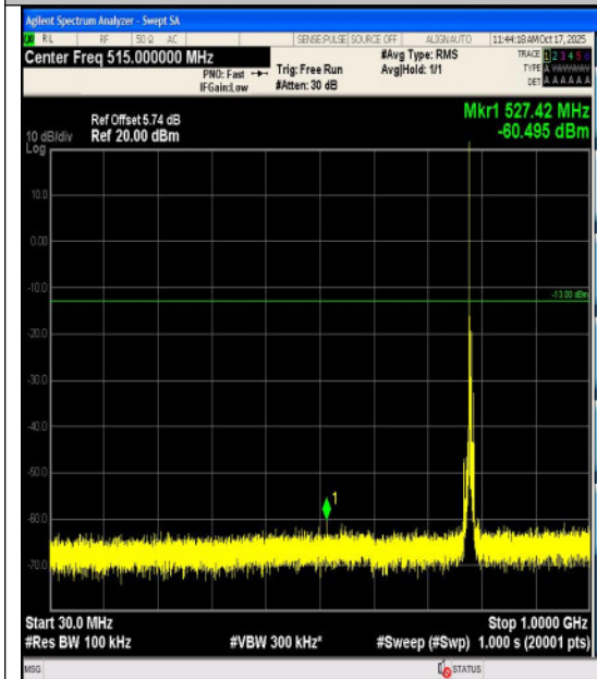
Band13-5MHz-QPSK-23255-1RB#0-3000~1000 0-PASS
