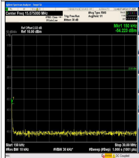
Band13-5MHz-QPSK-23255-1RB#24-1000~300 0-PASS
