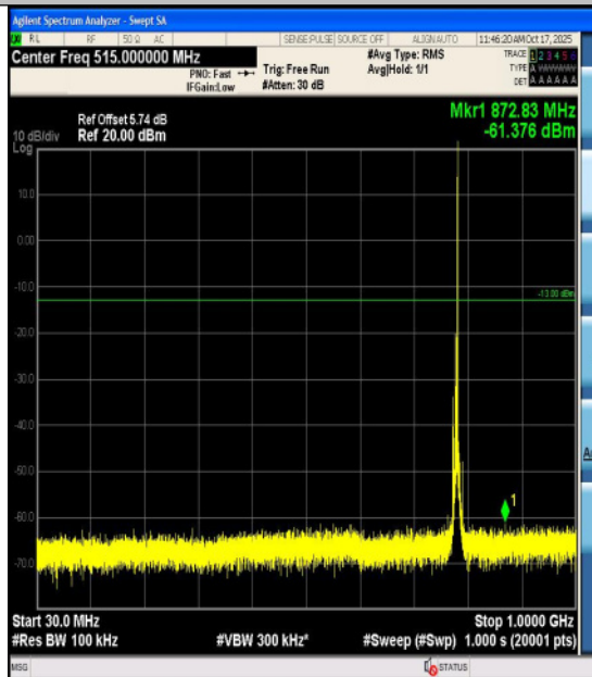
Band13-5MHz-QPSK-23255-1RB#24-3000~100 00-PASS
