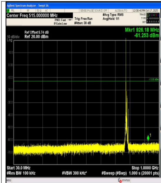
Band13-10MHz-QPSK-23230-1RB#0-3000~100 00-PASS
