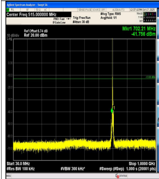
Band17-5MHz-QPSK-23755-1RB#0-3000~1000 0-PASS
