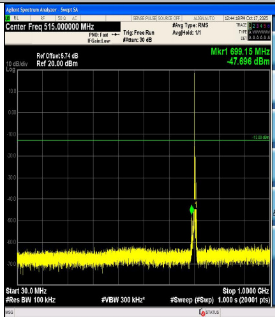
Band17-5MHz-16QAM-23790-1RB#0-3000~100 00-PASS
