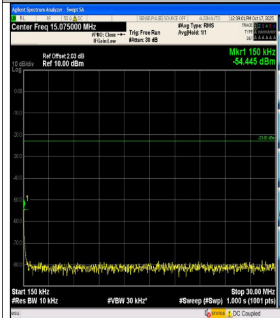
Band17-5MHz-QPSK-23755-1RB#24-1000~300 0-PASS
