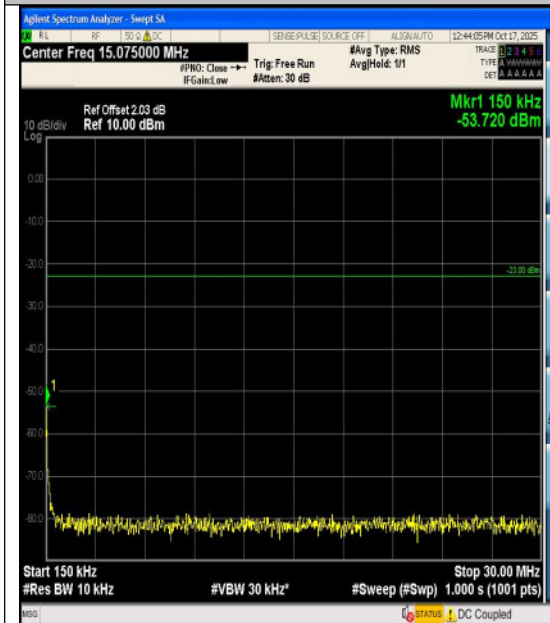
Band17-5MHz-16QAM-23790-1RB#0-1000~300 0-PASS
