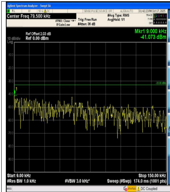
Band17-10MHz-16QAM-23790-1RB#49-30~100 0-PASS
