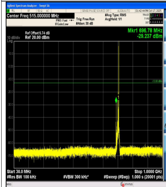
Band17-10MHz-16QAM-23790-1RB#49-3000~1 0000-PASS
