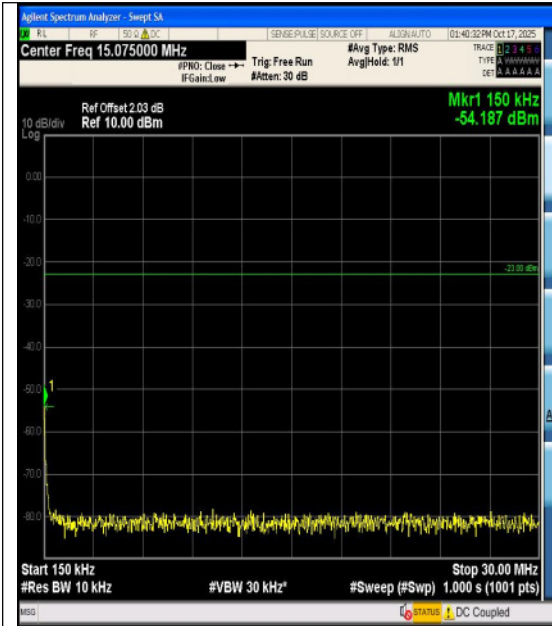
Band17-10MHz-16QAM-23790-1RB#0-1000~30 00-PASS
