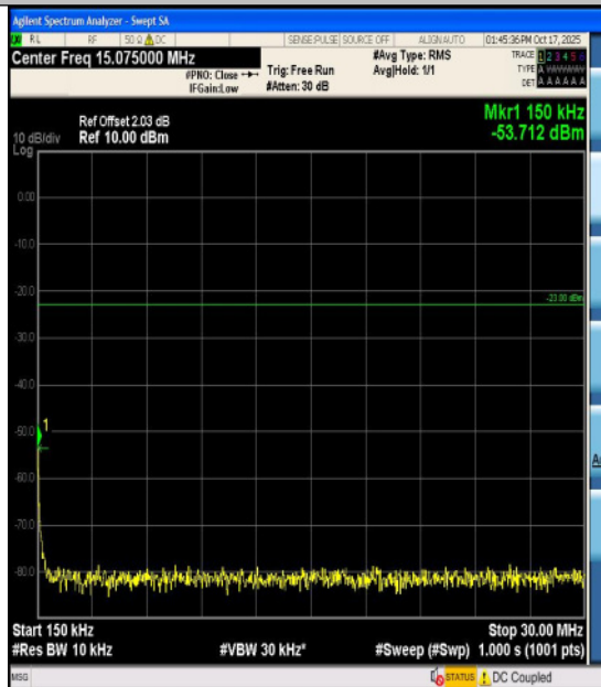
Band17-10MHz-QPSK-23800-1RB#0-1000~300 0-PASS
