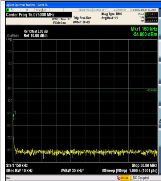
Band25-20MHz-16QAM-26590-100RB#0-1000~ 3000-PASS
