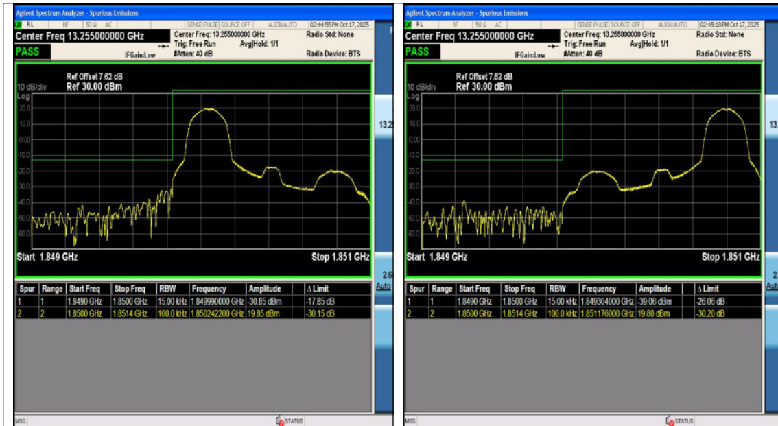
Band25-1.4MHz-QPSK-26047-6RB#0-PASS
