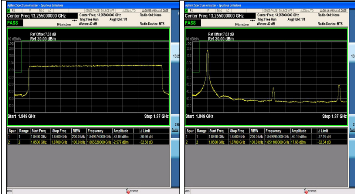
Band25-20MHz-16QAM-26140-1RB#99-PASS
