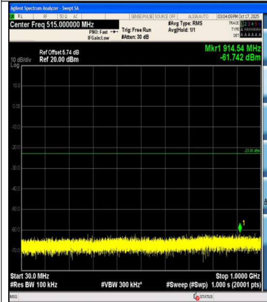
Band25-1.4MHz-QPSK-26683-6RB#0-3000~200- 00-PASS
