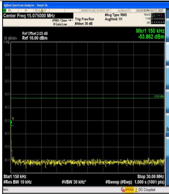
Band25-1.4MHz-QPSK-26683-6RB#0-1000~300- 0-PASS
