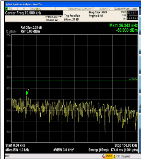
Band25-1.4MHz-QPSK-26365-1RB#0-30~1000- PASS
