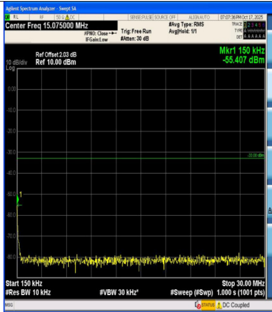
Band25-3MHz-16QAM-26055-1RB#14-1000~3000-PASS
