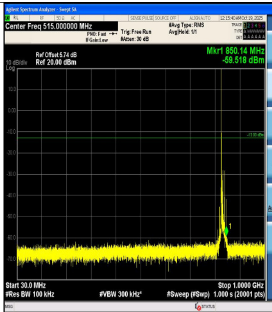
Band26(824-849)-15MHz-16QAM-26915-1RB#0 -3000~10000-PASS
