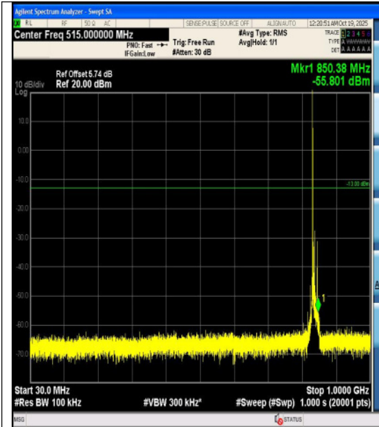
Band26(824-849)-15MHz-QPSK-26965-1RB#0-3 000~1000-PASS
