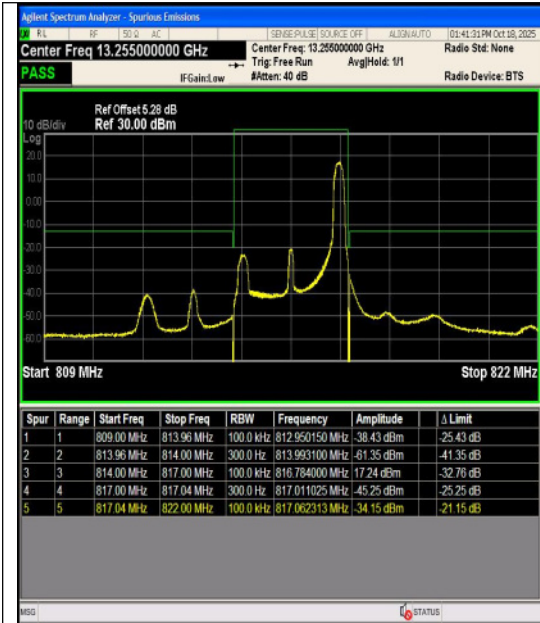
Band26(814-824)-3MHz-QPSK-26775-1RB#0-PA
