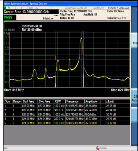
Band26(814-824)-3MHz-16QAM-26775-1RB#0-P
