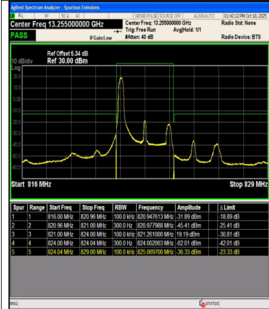
Band26(814-824)-3MHz-QPSK-26775-15RB#0-P
